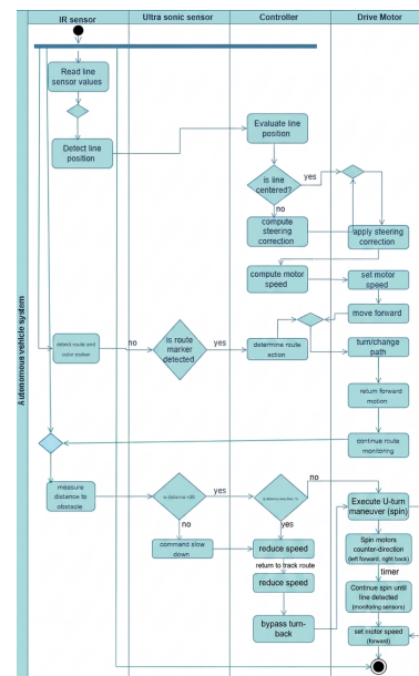
Fig. 3. Activity Diagram
